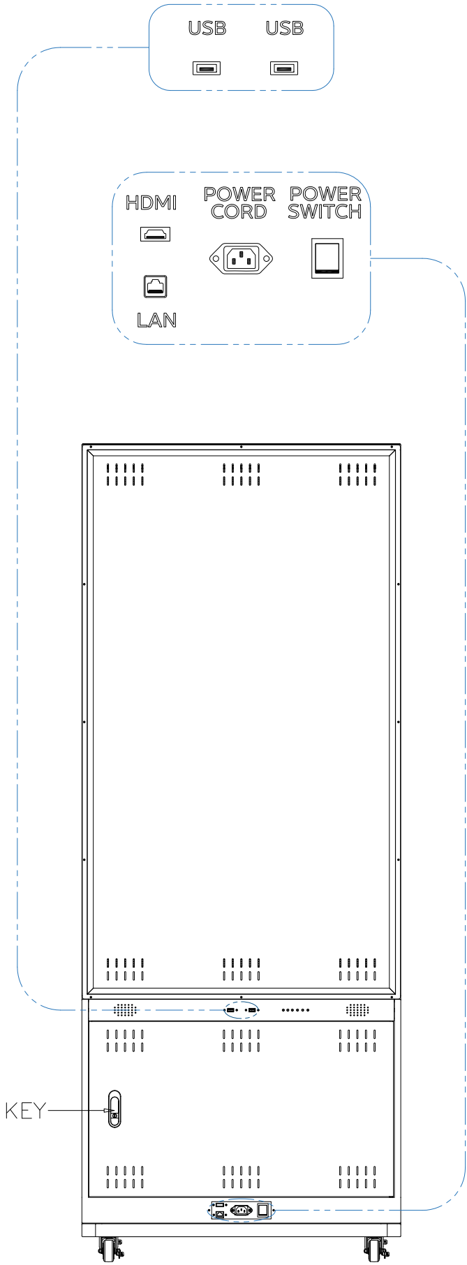
REAR VIEW
