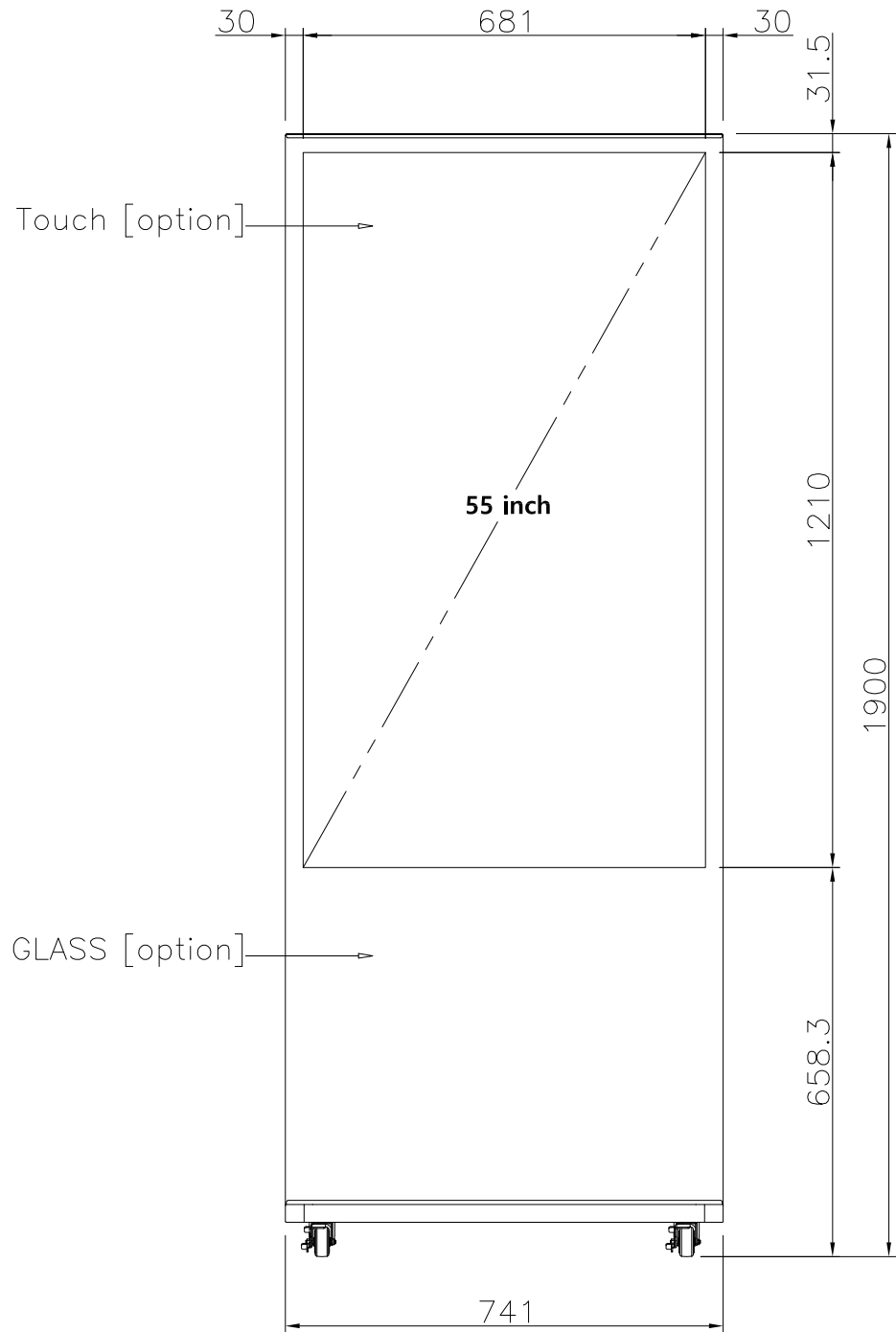
FRONT VIEW
